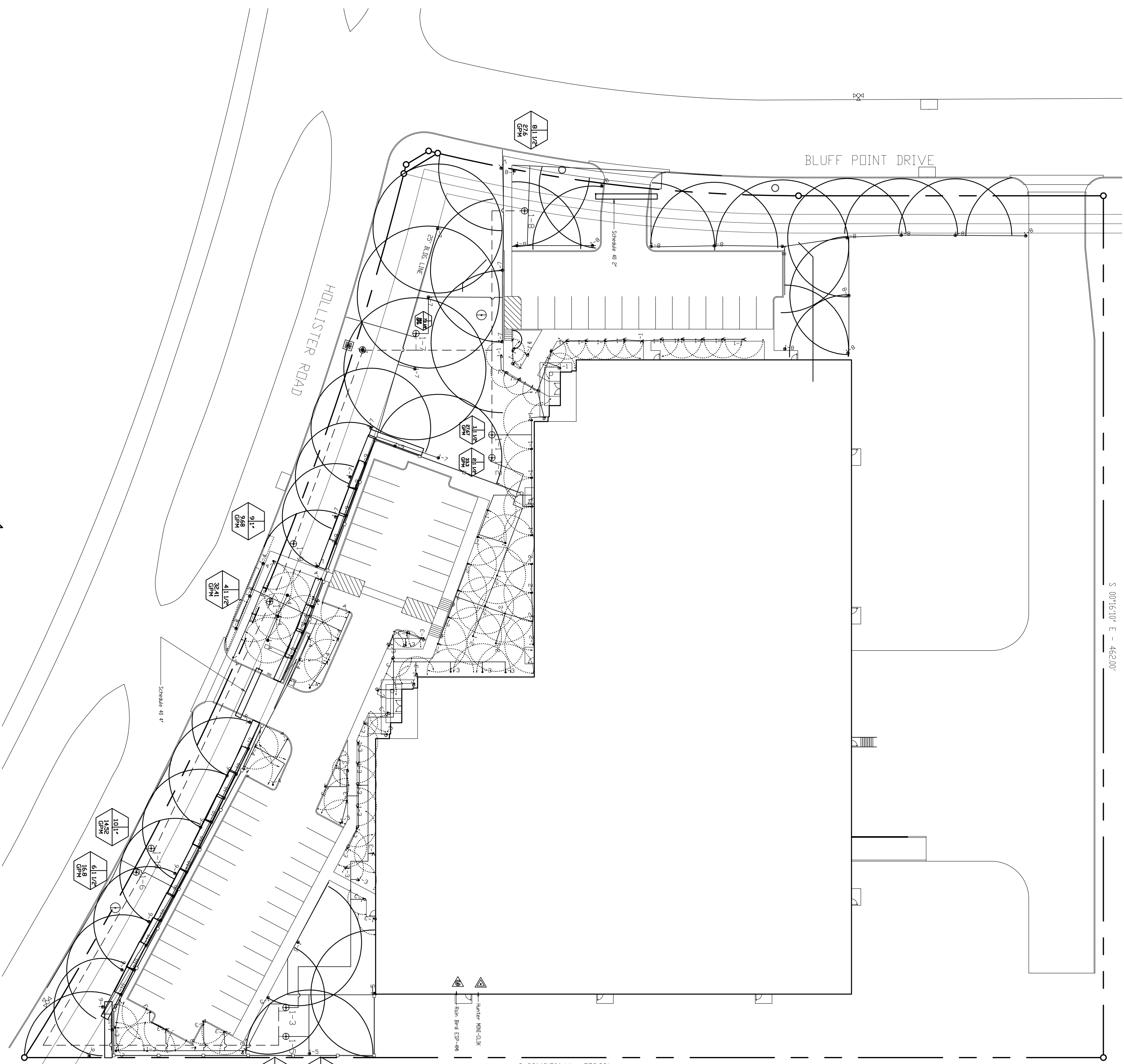
SITE PLAN 1" = 30'-0"
